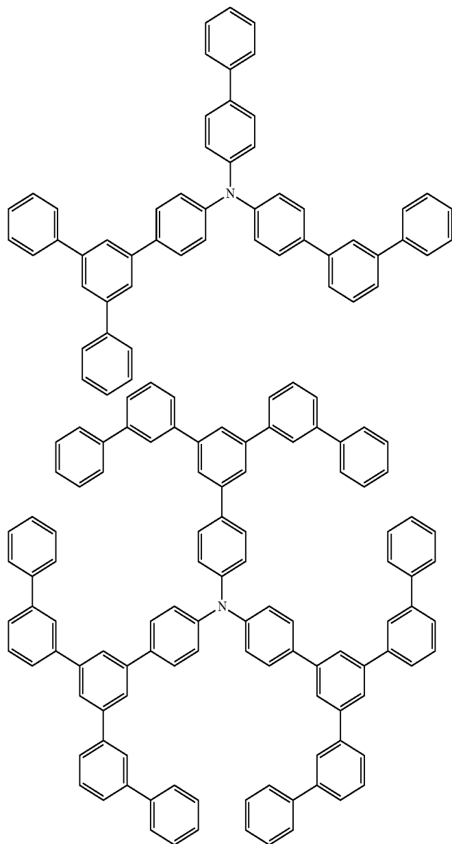
[Chem 24]
