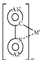
[Chem 36]
